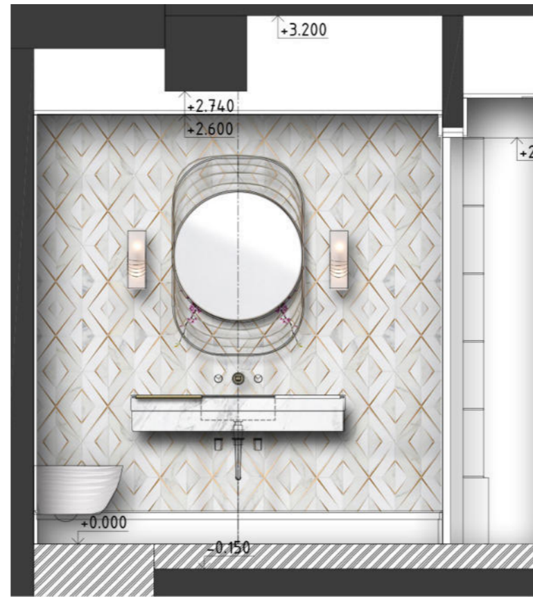
ELEVATION D
